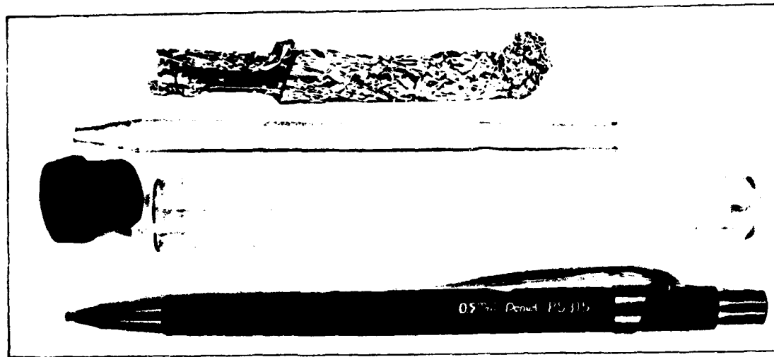
PLATE 6. CHROMOSORB TUBE, ALUMINUM FOIL WRAP, AND STORAGE TUBE. PENCIL ADDED FOR SCALE. CHROMOSORB MATERIAL IN LEFT 1/3 OF TUBE
